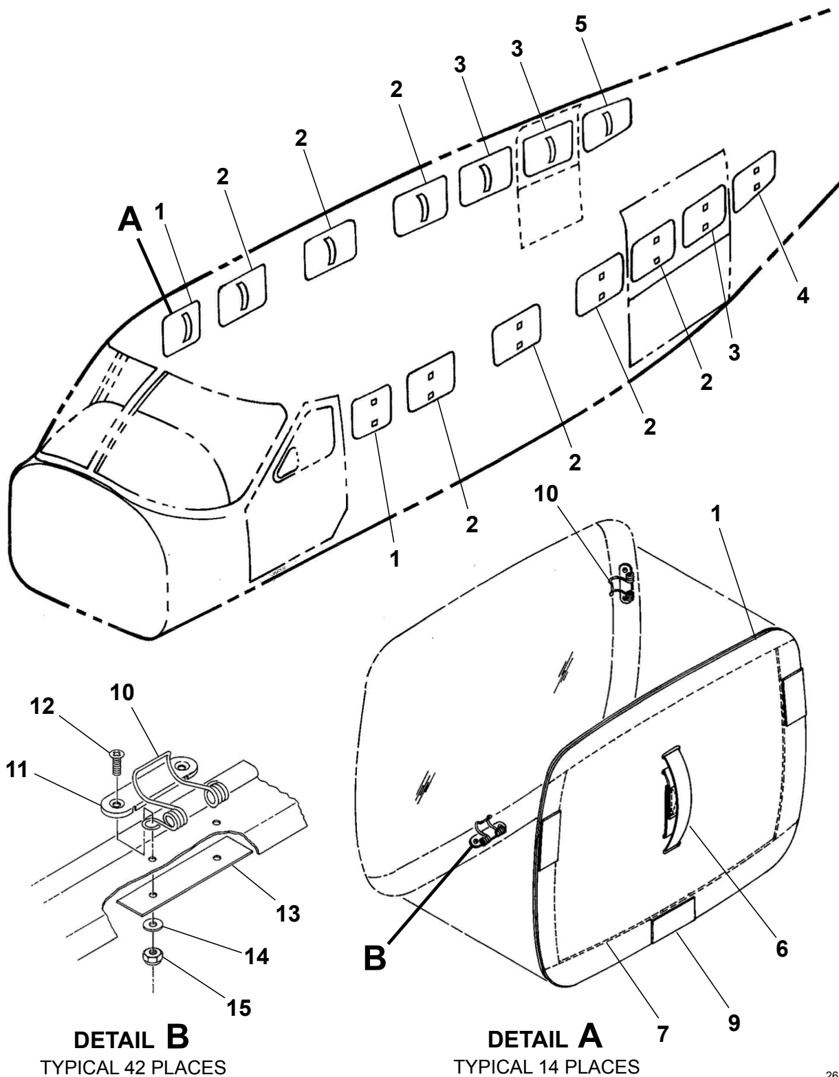
WINDOW PLUG INSTALLATION - PASSENGER VERSION Figure 02. (Sheet 1)
