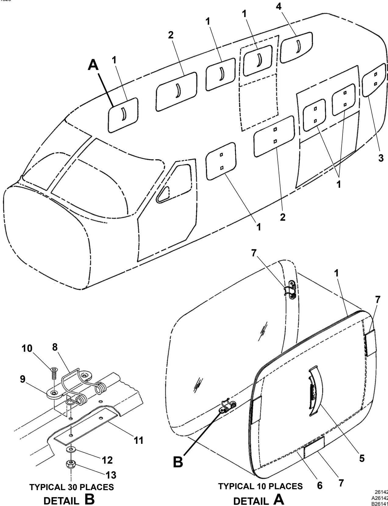
WINDOW PLUG INSTALLATION Figure 01. (Sheet 1)
