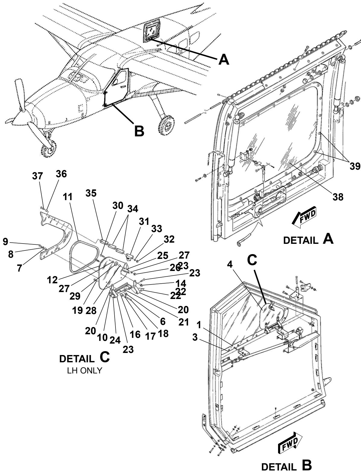
CREW AND PASSENGER DOOR WINDOWS Figure 01. (Sheet 1)
